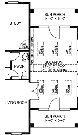
Partial First Floor Plan w/ Opt. Solarium
