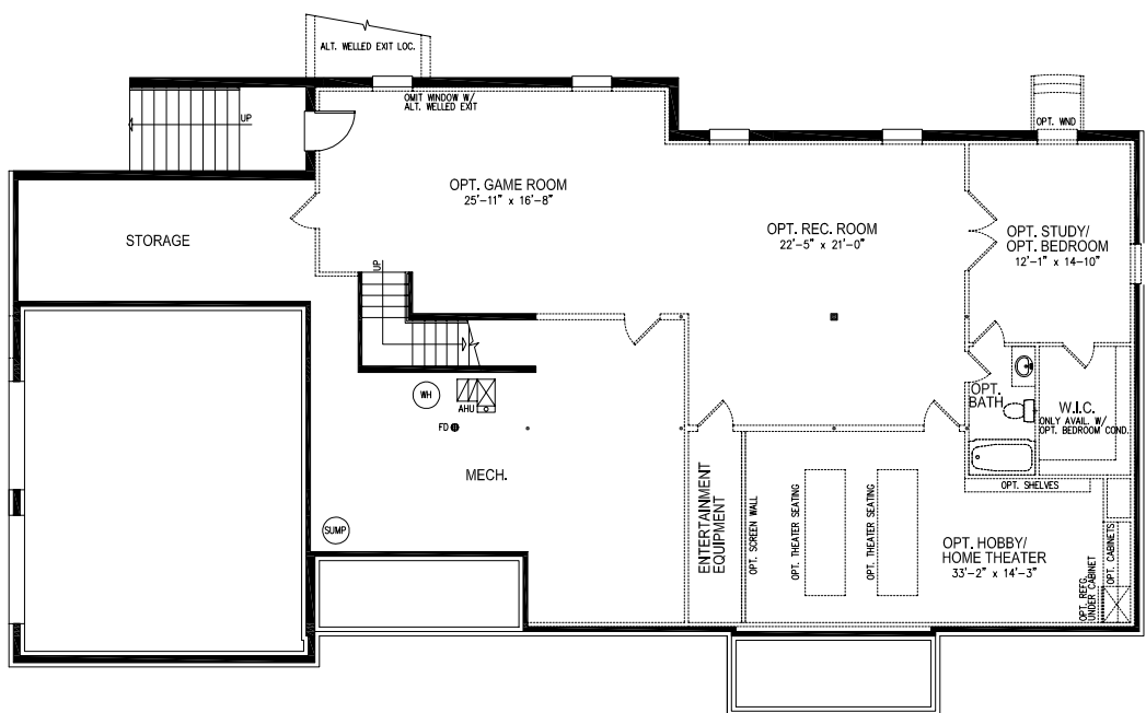
Foundation Plan – Inground Condition
