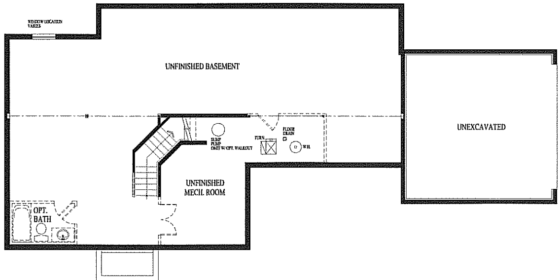
Partial Fnd. Plan w/ Opt. Single Door at Walk-out Cond.
