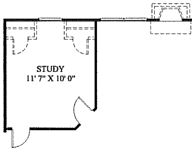
Partial Floor Plan w/ Opt. Extended Study/Bed
