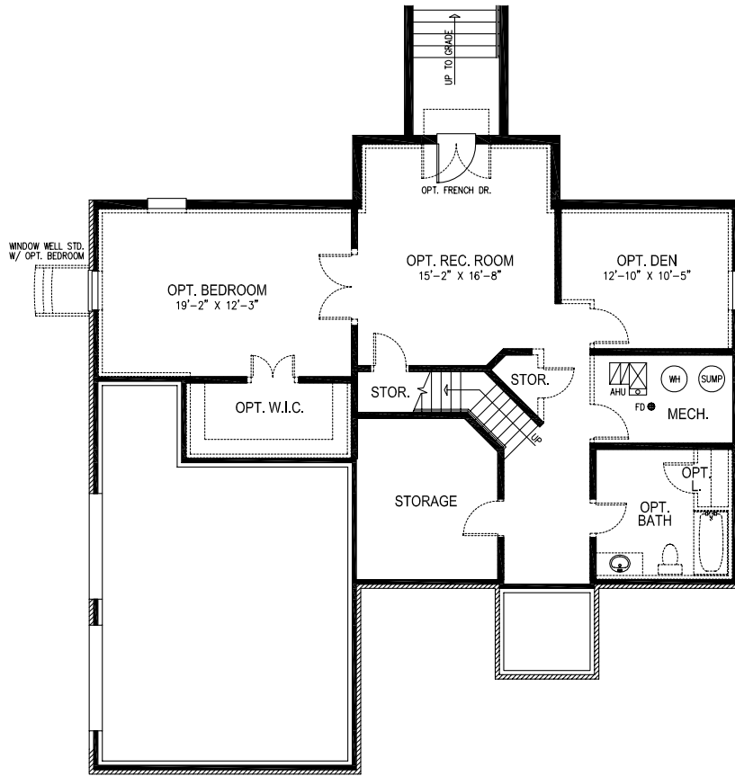
Foundation Plan – Inground Condition
