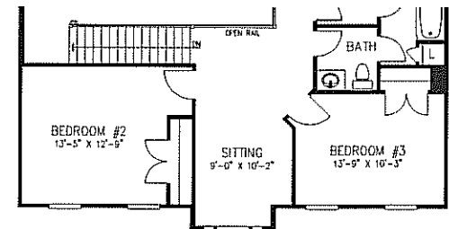
Alt. Second Floor Plan w/ Sitting
