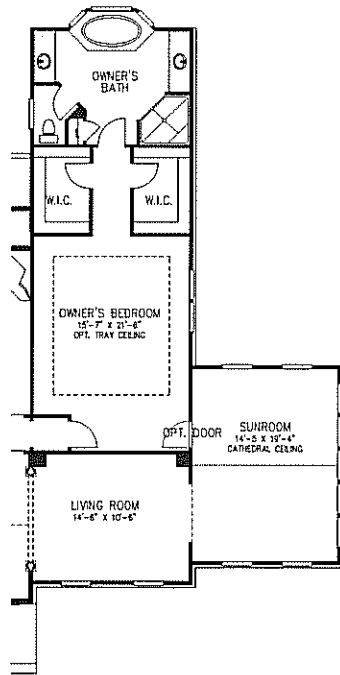
Partial First Floor Plan w/ Opt. Extended Master Bedroom & Opt. Side Sunroom
