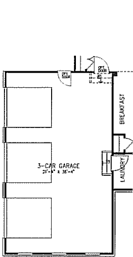
Partial First Floor Plan w/ Opt. 3-Car Garage
