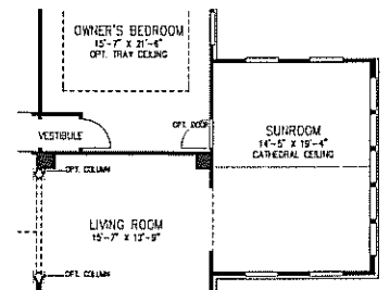
Opt. Side Sunroom Floorplan
