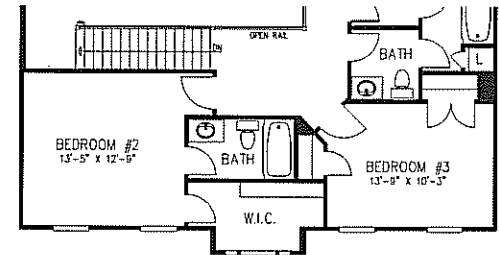
Alt. Second Floor Plan w/ Bath
