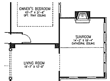
Opt. Side Sunroom Floorplan w/ Fireplace
