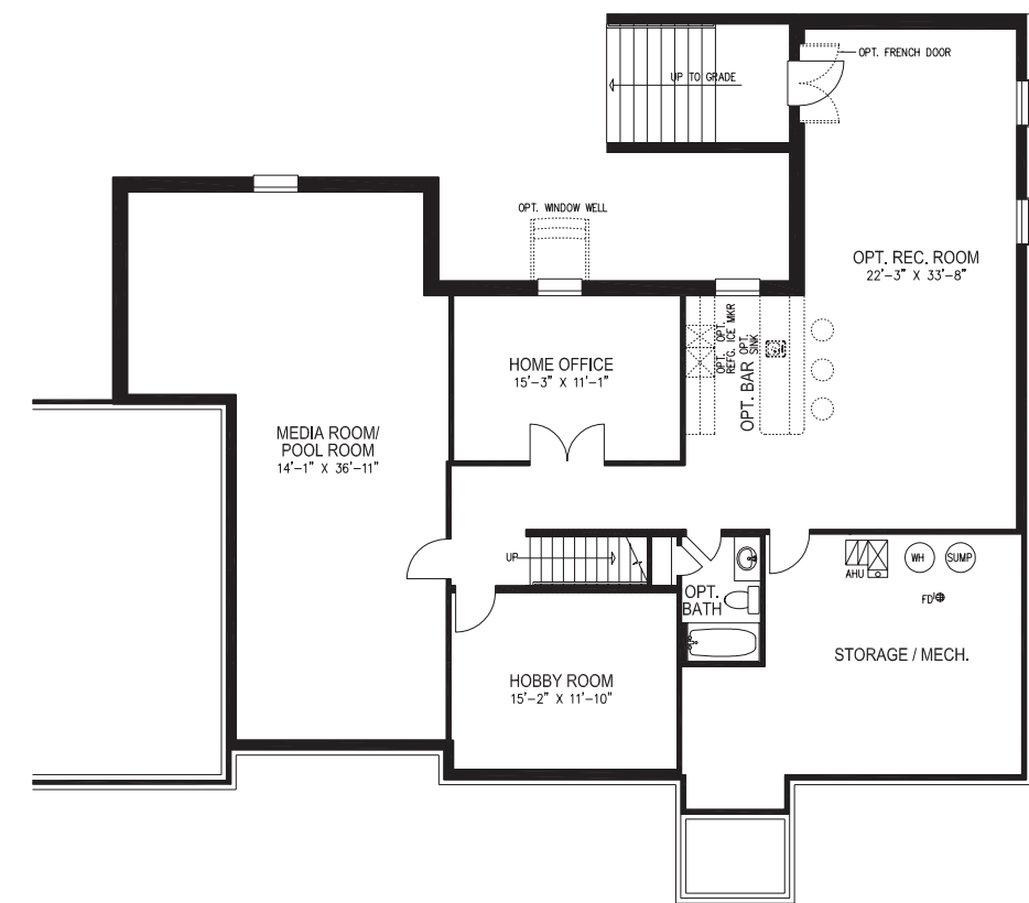
Foundation Plan – Inground Condition
