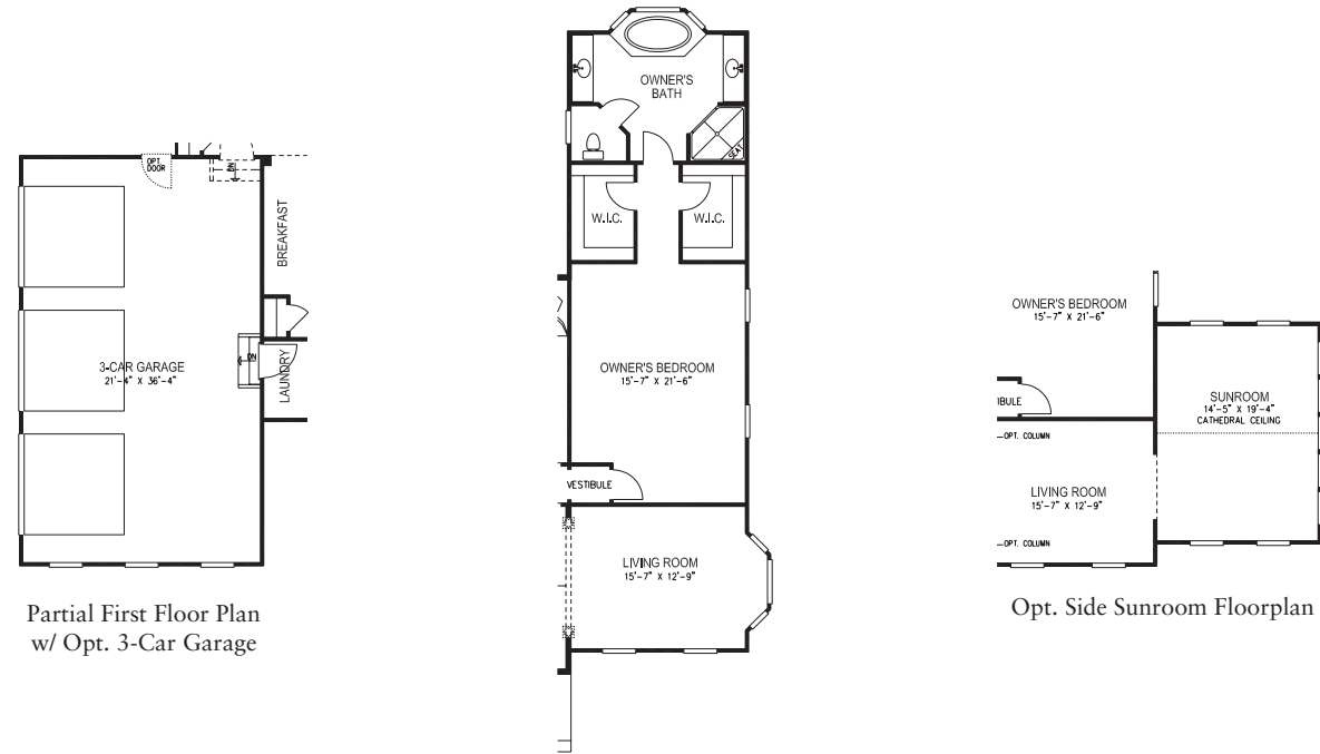
Partial First Floor Plan w/ Opt. Extended Master Bedroom
