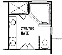
PARTIAL FIRST FLOOR PLAN W/ OPT. LUXURY MASTER BATH
