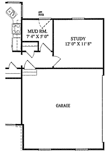
Partial First Floor Plan w/ Opt. Study / Mud Room
