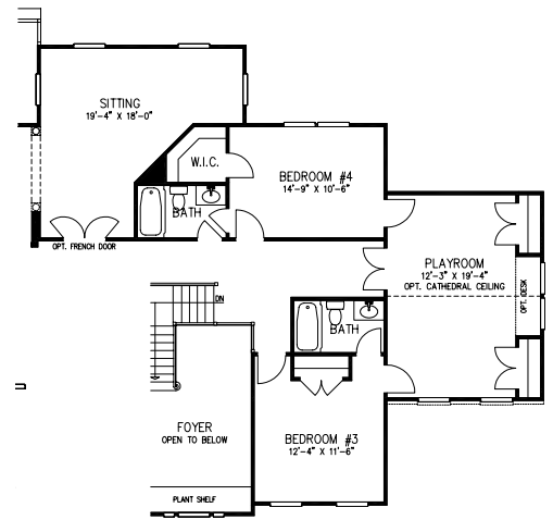
Partial Second Floor Plan w/ Side Sunroom (2-Story) Version #1
