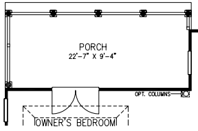
Partial Second Floor Plan w/ Opt. Covered Porch
