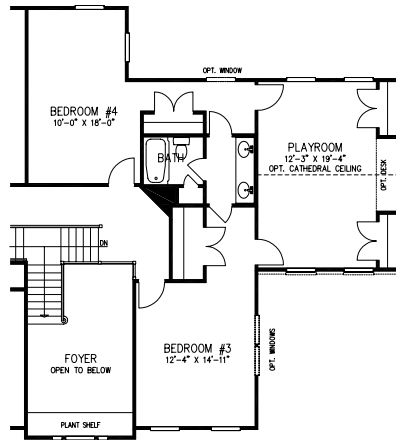
Partial Second Floor Plan w/ Side Sunroom (2-Story) Version #2
