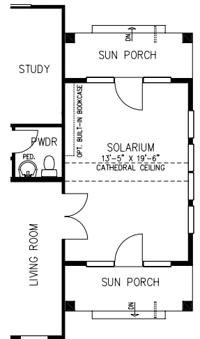
Partial First Floor Plan w/ Opt. Solarium
