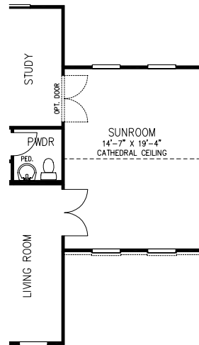
Partial First Floor Plan w/ Side Sunroom (1-Story)
