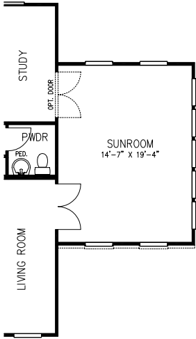
Partial First Floor Plan w/ Side Sunroom (2-Story) Version #1
